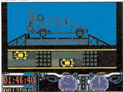
Super Scramble.
